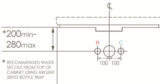
PLUMBING ROUGH-IN
